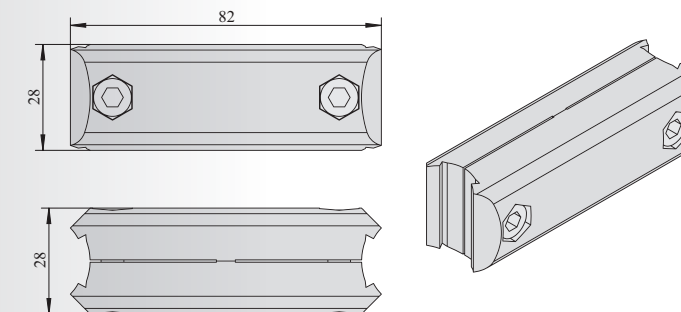
平行加长接头 Parallel Extension Connector
