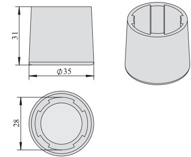
线棒脚套 Frame Foot Cover
