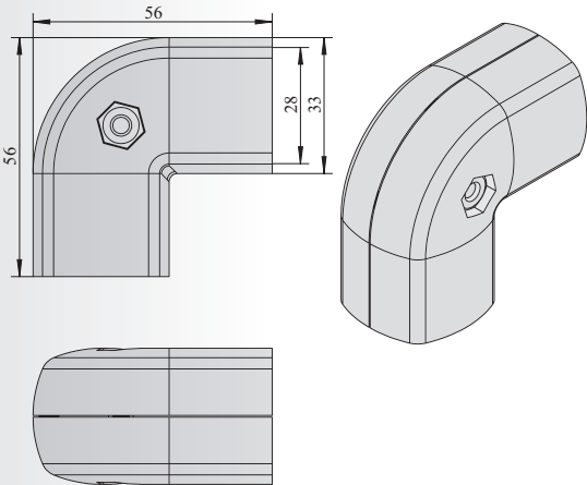
90° 外接头 Connector Outer Type 90°
