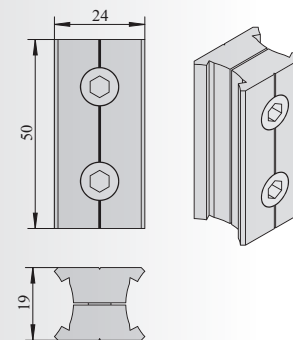
平行固定接头 B-L50 Parallel Fixed Connector B-L50
