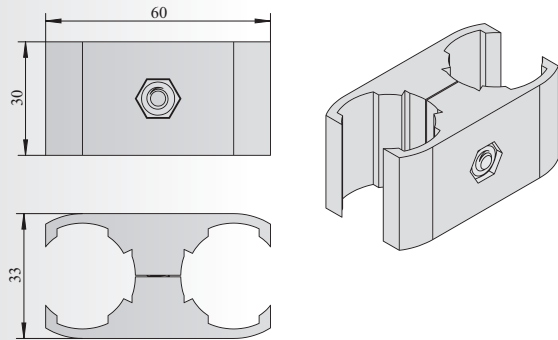
平行外抱接头 Parallel External Holder Connector
