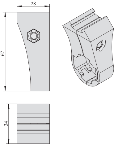
扶手接头 Armrest Joint
