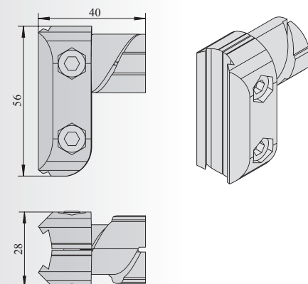
加强内直接头 Reinforced Connector Inner Vertical Type
