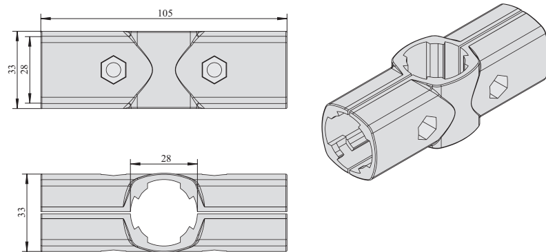
外抱十字接头 Cross Connector Vertical Type
