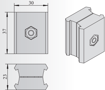
平行固定接头 A Parallel Fixed Connector A
