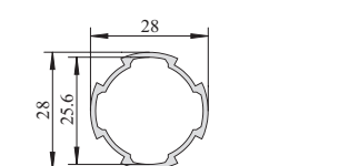
薄壁基础线棒 Thin Wall Foundation Frame
