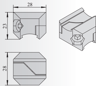
90° 交叉接头 90° Cross Connector
