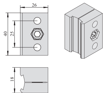
双孔功能附件 Dual-hole Functional Accessories
