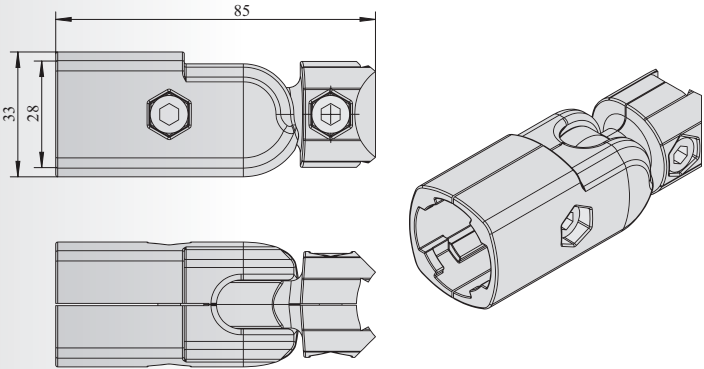
90° 活动外接头 Free Connector Outer Type 90°
