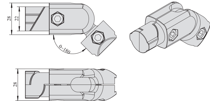
180° 固定外接头 Fixed Connector Outer Type 180°
