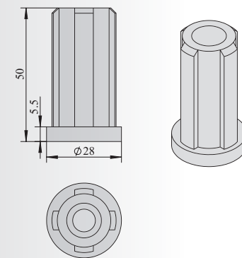
一体式固定脚座 Integrated Fixed Foot Connector
