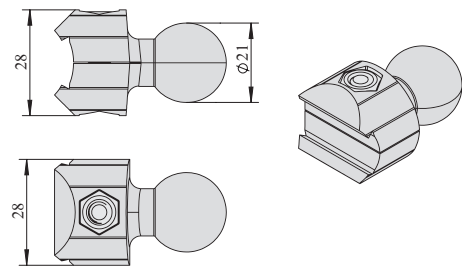
圆头挂钩 Round Nose Hook
