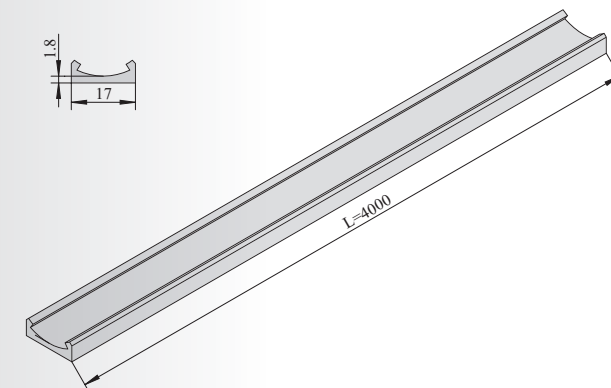
平面防磨卡扣 Flat Anti-wear Buckle
