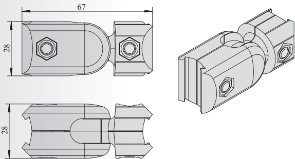
多角度固定接头 Multi-angle Fixed Connector
