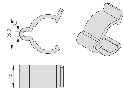
吊牌卡扣 Hangtag Clip
