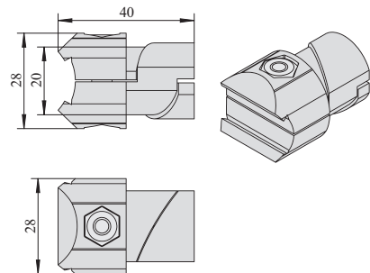
内直旋转接头 Connector Inner Rotate Type
