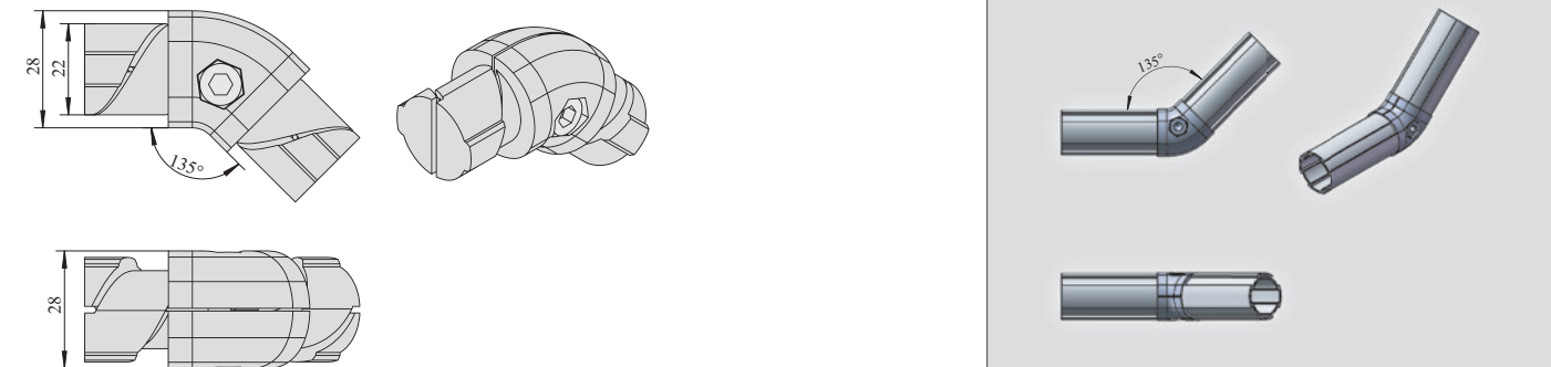
135° 内接头 Connector Inner Type 135°
