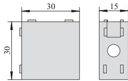
1530 门角件 1530 Connection block
