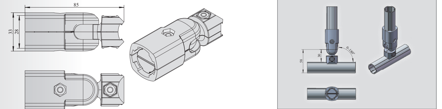
180° 固定内接头 Fixed Connector Inner Type 180°
