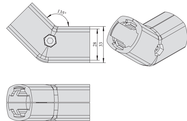
135° 外接头 Connector Outer Type 135°
