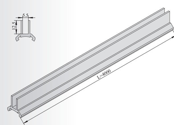
5.3MM 面板卡槽 5.3MM Panel Holder
