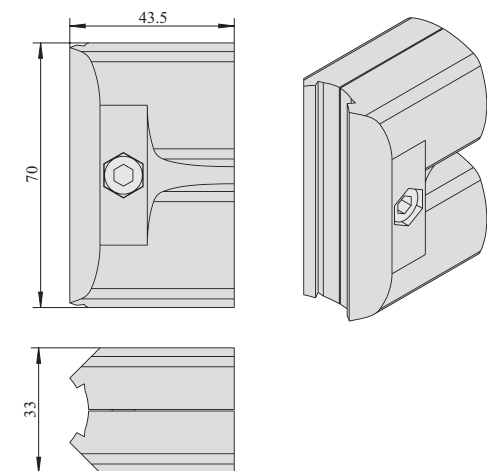
双管外直接头 Multi Connector Outer Type (Double Pipes)
